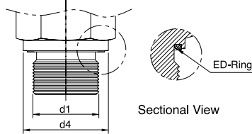
Form E (DIN 3852 Part 11) With sealing by DIN 3869 ring seals (* ED-Ring)
