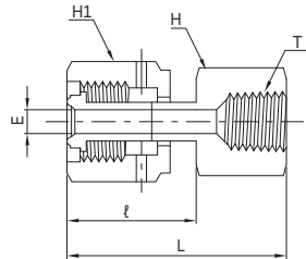
Swivel Tube Fitting Connector
