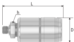
Male BSPP
